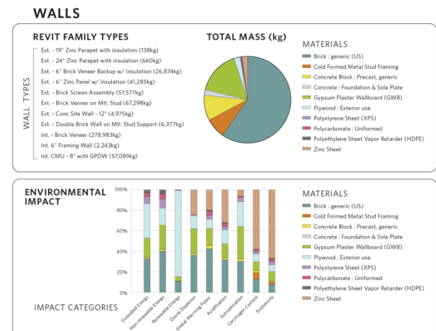
Figure 5: This assessment of wall types in the design of Building 7R shows the relationship between Revit family types, material breakdowns by weight, and environmental impacts.
